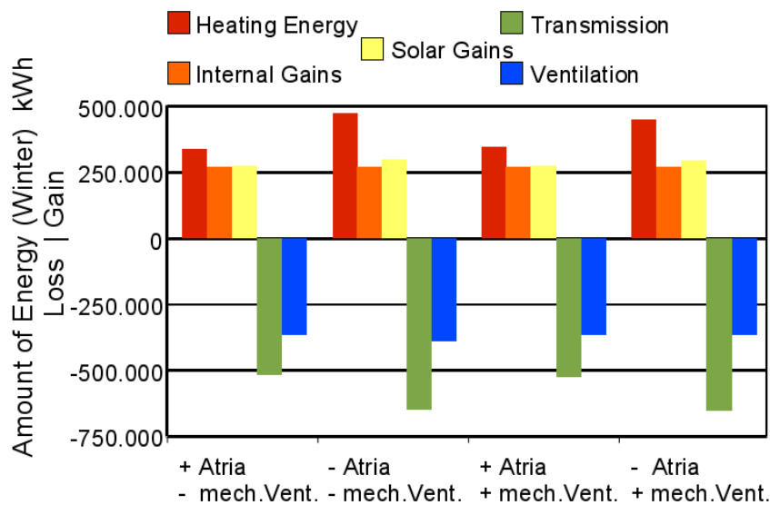
Figure 7 Energy Balance for the Winter Period of the Building with/without Atria and with/without Mechanical Ventilation
