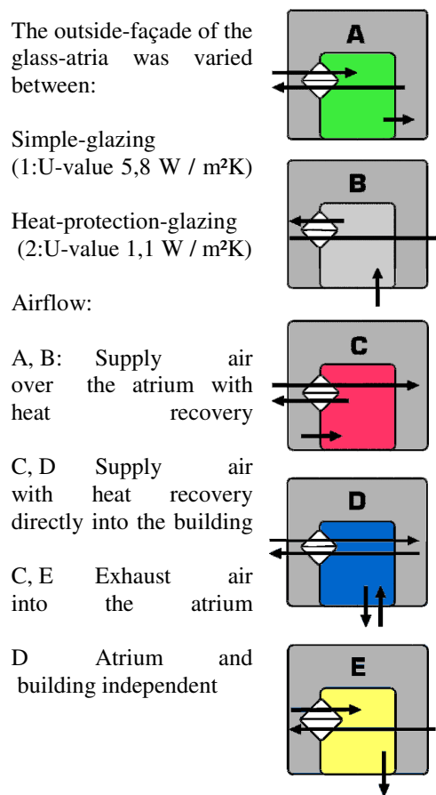
Figure 3: Variation of the Airflow into an Atrium
